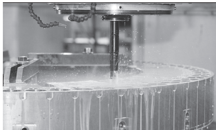
GP Meccanica etxearen 3000 Premium Plus Five makina. | FAGOR AUTOMATION
